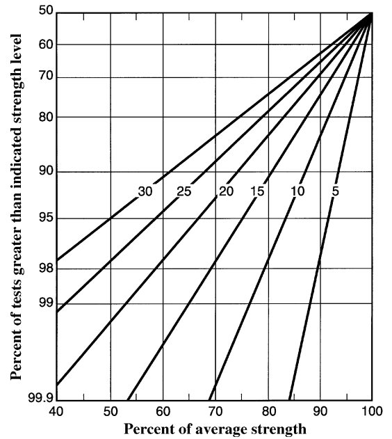
Fig. 3.4—Cumulative distribution curves for different coefficients of variation.
