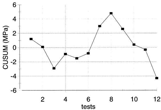
Fig. A.4—CUSUM chart with partial data.
